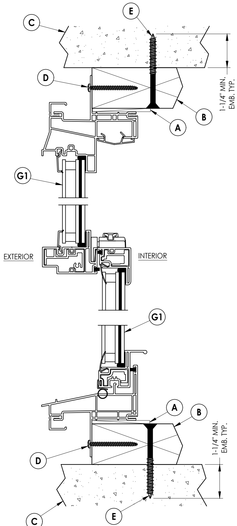
3 VERTICAL CROSS SECTION 2 Shown w/ 2X Buck Construction
