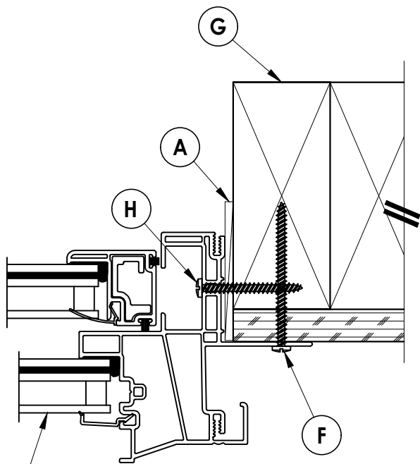
2 HORIZONTAL CROSS SECTION 2 Shown w/ 2X Stud Construction
